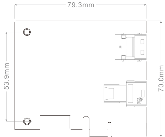
Standard PCIe from factor
